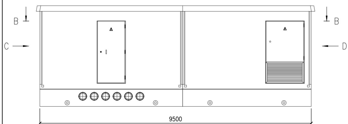
VISTA FRONTAL
